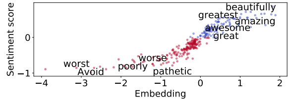
Figure 1: IMDB: remaining embedding component vs sentiment score ( (\#pos. - \#neg.) / \#all texts with the word).
