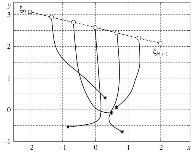
Fig. 1. Protocol (3) for the agents with damping velocity feedback ( a = 2 ).
