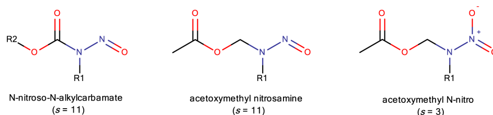
Figure 7. Three toxicophores generalized by MF_87.
