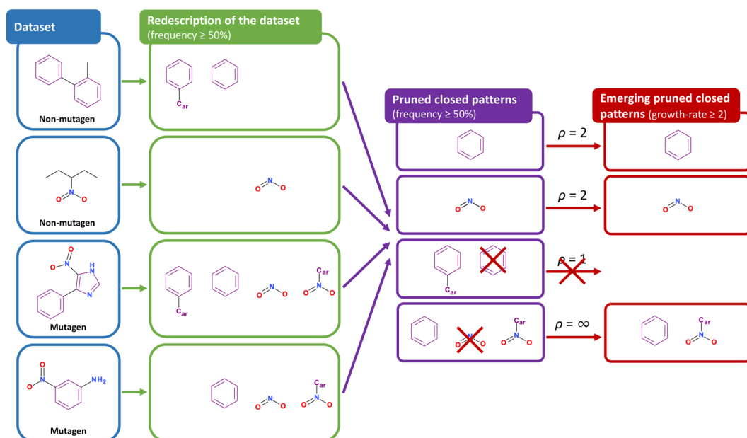
Figure 2. Illustration of going from a set of molecules to emerging pruned closed patterns.
